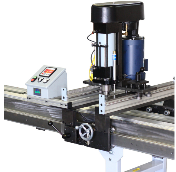
2-axis drilling machine
