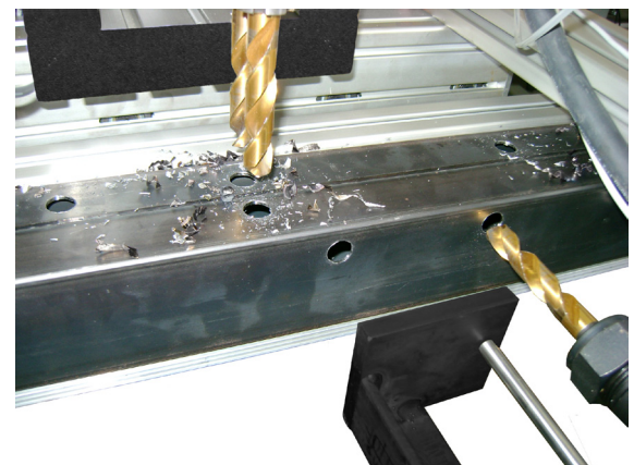
KDP multi-axis drill - vertical and horizontal
