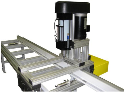
KDP multi-axis drill – vertical and horizontal
