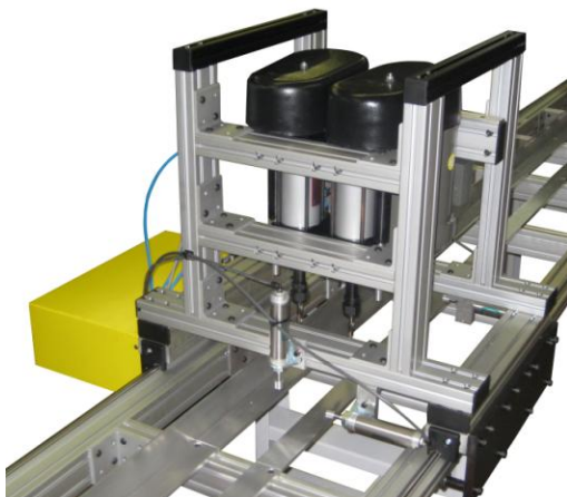
KDP multi-head drill - vertical
