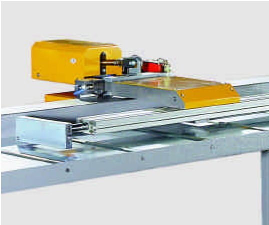
PDE stop with RC conveyor & metal inserts
